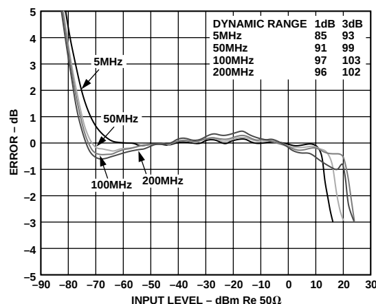
Figure 32. Log Linearity vs. Input Level at T_A = +25^{\circ}\text{C} , for Frequencies of 5 MHz, 50 MHz, 100 MHz and 200 MHz
