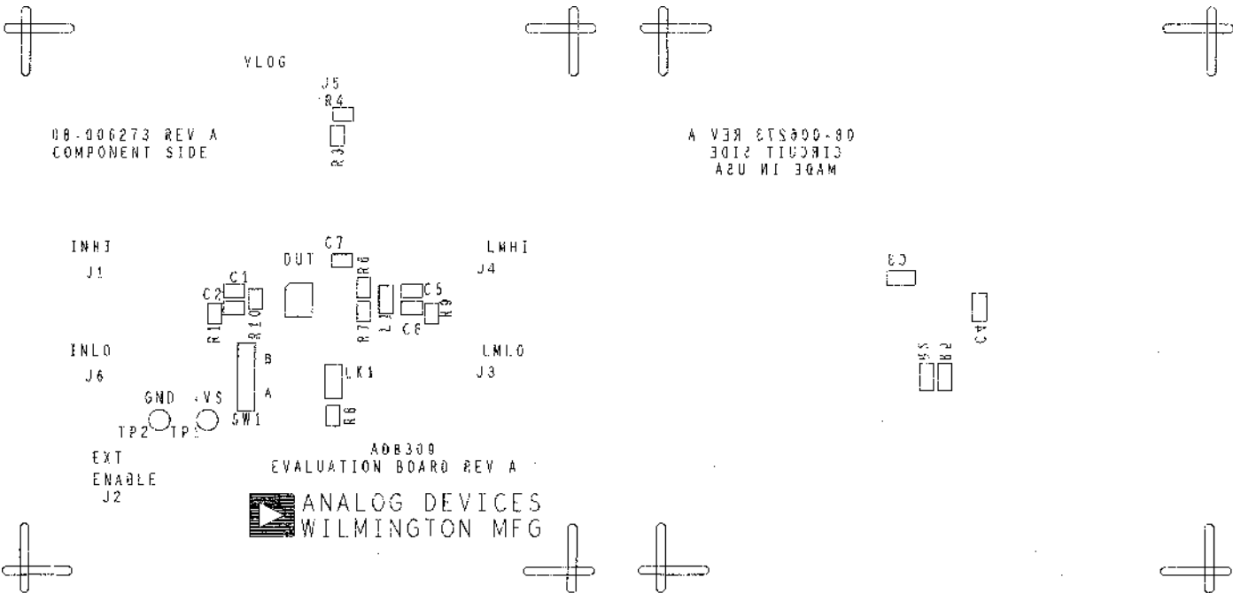
Figure 43. Signal Layer Silkscreen
