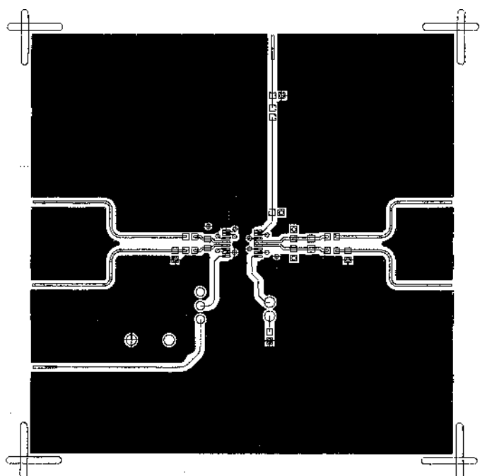
Figure 41. Layout of Signal Layer
