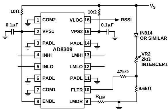
Figure 36. Trimming Intercept to -113 \text{ dBV} \pm 4 \text{ dB}
