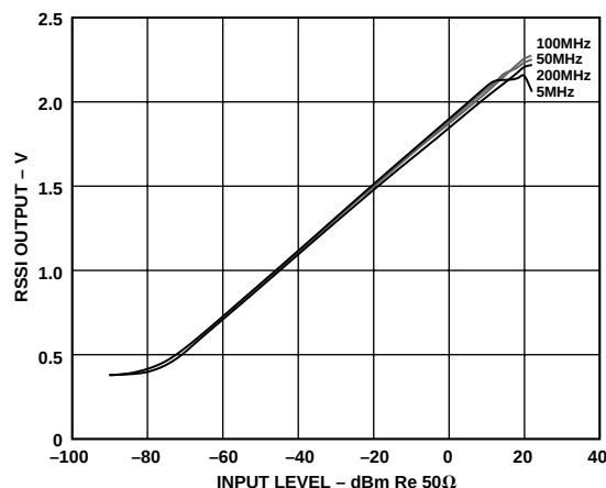
Figure 31. RSSI Output vs. Input Level at T_A = +25^{\circ}\text{C} , for Frequencies of 5 MHz, 50 MHz, 100 MHz and 200 MHz
