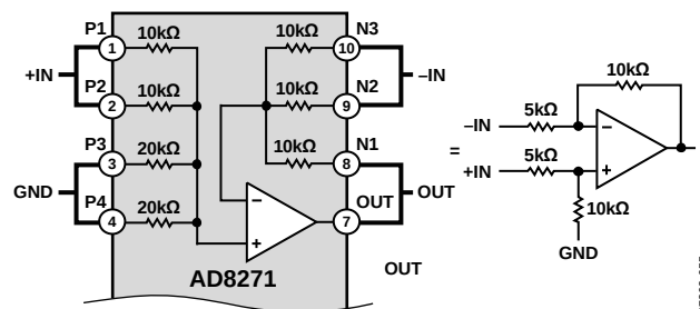
Figure 47. Gain = 2 Difference Amplifier, Referenced to Ground
