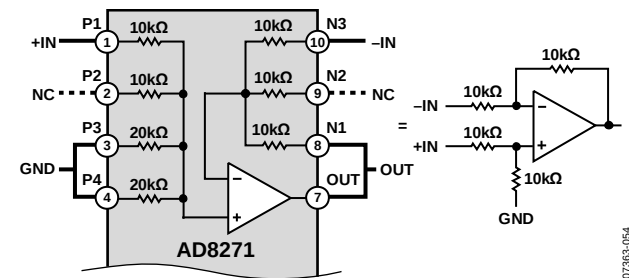
Figure 46. Gain = 1 Difference Amplifier, Referenced to Ground
