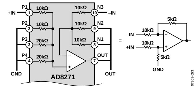
Figure 45. Gain = 1/2 Difference Amplifier, Referenced to Ground
