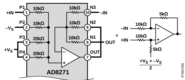
Figure 48. Gain = 1/2 Difference Amplifier, Referenced to Midsupply
