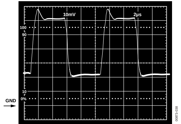
Figure 37. V_S = 5\text{ V} , 0\text{ V} ; Gain-of-2 Inverter Response to 20\text{ mV} Step, Centered 20\text{ mV} Below Ground
