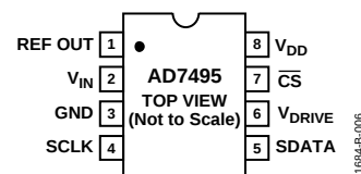
Figure 6. AD7495 SOIC/MSOP Pin Configuration
