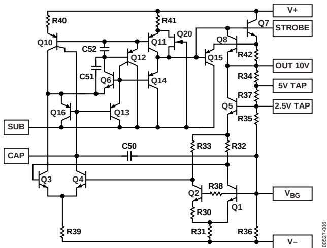
Figure 5. Schematic Diagram
