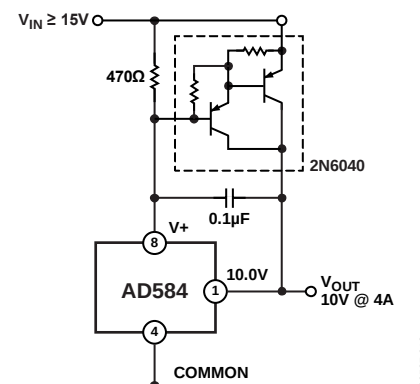
Figure 12. High Current Precision Supply
