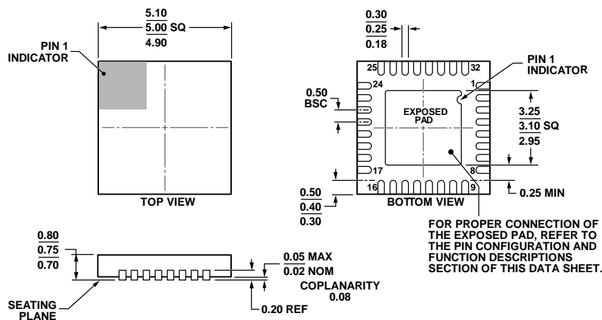
COMPLIANT TO JEDEC STANDARDS MO-220-WHHD. Figure 57. 32-Lead Lead Frame Chip Scale Package [LFCSP_WQ] 5 mm x 5 mm Body, Very Very Thin Quad (CP-32-7) Dimensions shown in millimeters
