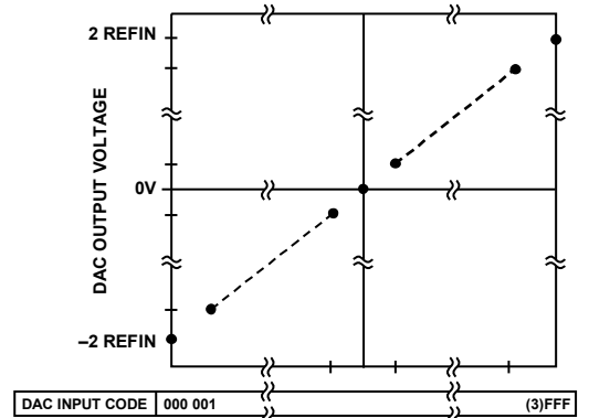
Figure 22. Output Voltage vs. DAC Input Codes (Hex)
