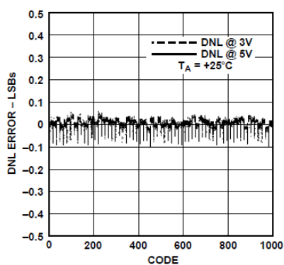
Figure 6. Typical DNL
