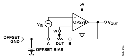
Figure 31. Noninverting Gain
