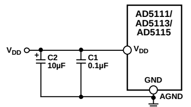
Figure 46. Power Supply Bypassing
