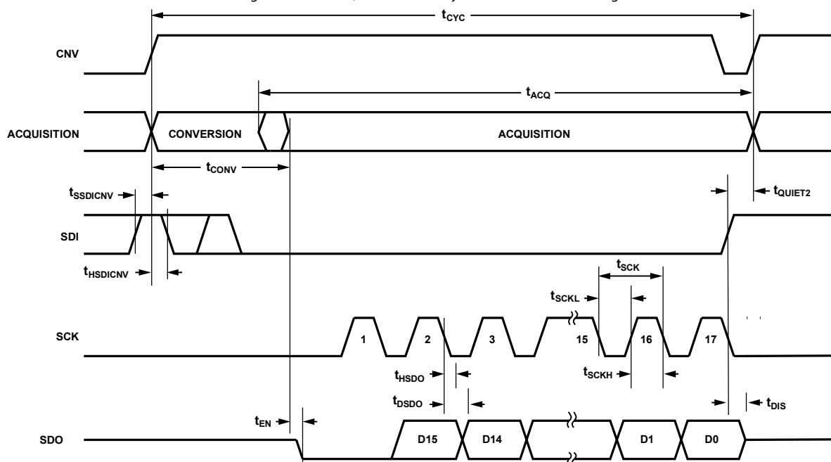
Figure 63. \overline{CS} Mode, 4-Wire with Busy Indicator Serial Interface Timing Diagram (Status Bits Not Shown)
