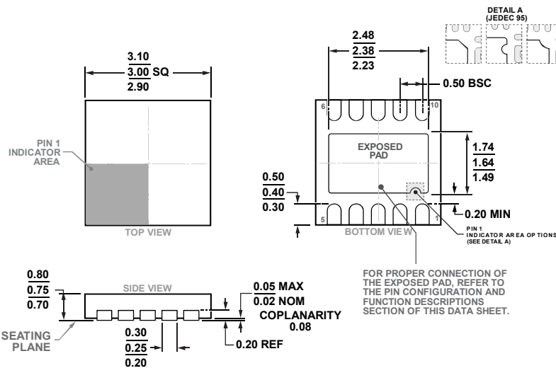
Figure 69. 10-Lead Lead Frame Chip Scale Package [LFCSP] 3 mm × 3 mm Body and 0.75 mm Package Height (CP-10-9)
