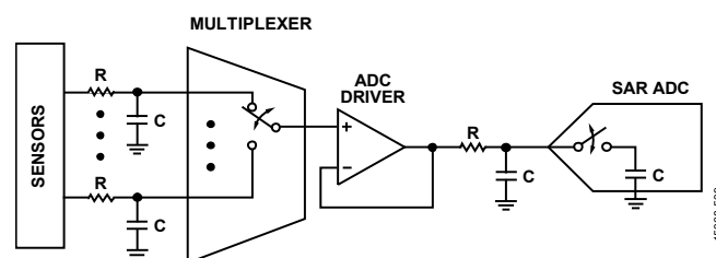
Figure 44. Multiplexed Data Acquisition Signal Chain Using the AD4001/AD4005
