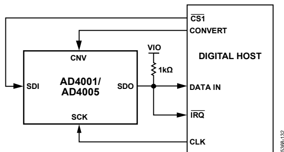
Figure 62. \overline{CS} Mode, 4-Wire with Busy Indicator Connection Diagram
