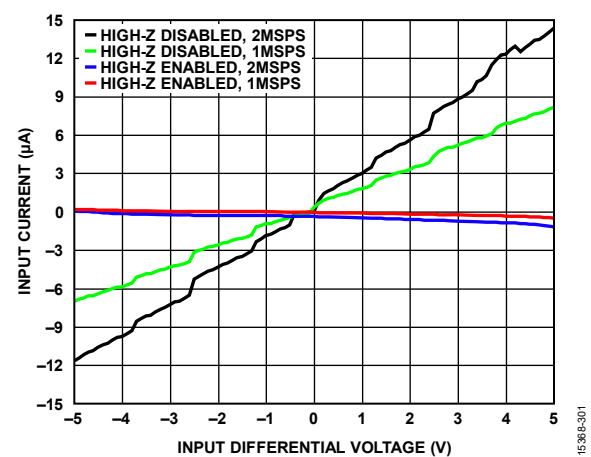
Figure 28. Analog Input Current vs. Input Differential Voltage
