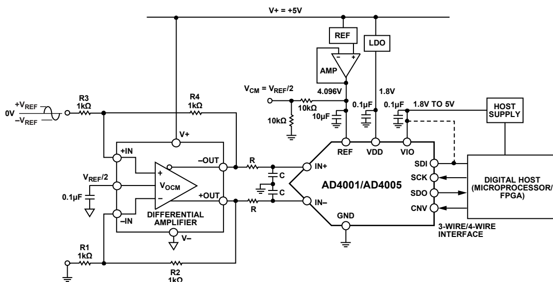
Figure 43. Typical Application Diagram for Single-Ended to Differential Conversion with a Fully Differential Amplifier
