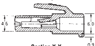
Section X-X
