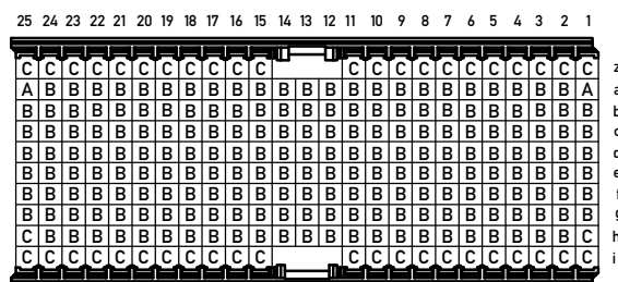
Board hole pattern (Component mounting side)
