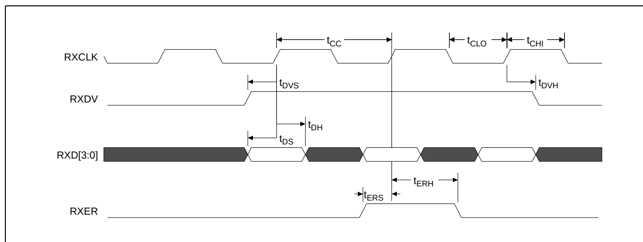
Figure 33 - MII Receive Timing Diagram
