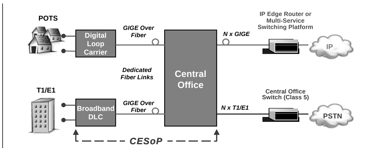
Figure 12 - Digital Loop Carrier using CESoP
