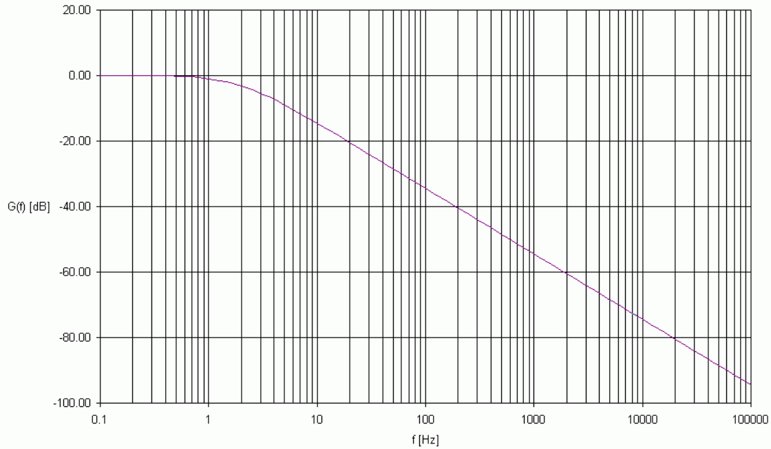
Figure 23 - Jitter Transfer Function
