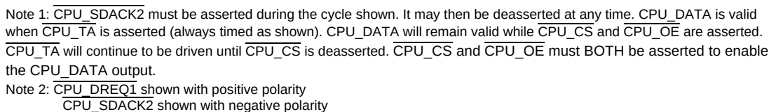
Figure 42 - CPU DMA Read - MPC8260
