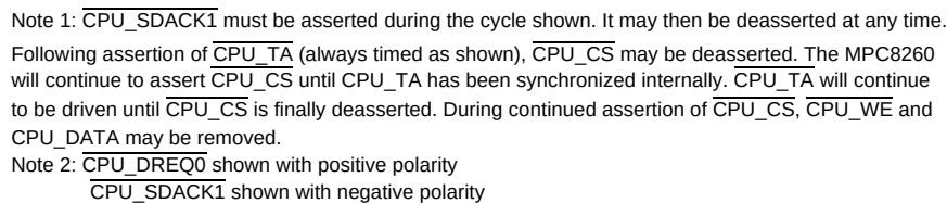
Figure 43 - CPU DMA Write - MPC8260
