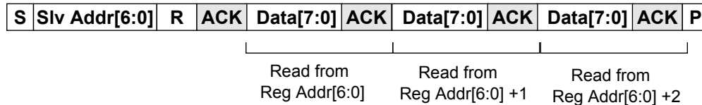
Figure 27 - I 2 C Data Read Burst Mode
