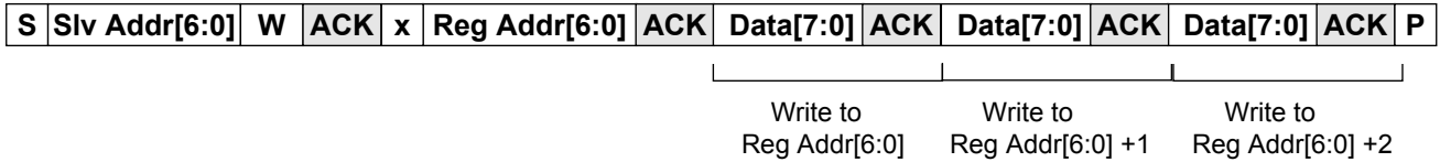
Figure 26 - I 2 C Data Write Burst Mode
