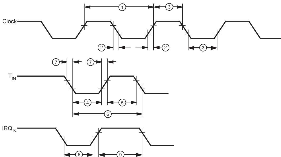
Figure 8. AC Electrical Timing
