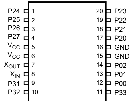
Figure 5. 20-Pin SSOP Pin Configuration, STANDARD Mode
