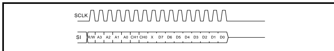
FIGURE 7. SPI WRITE
