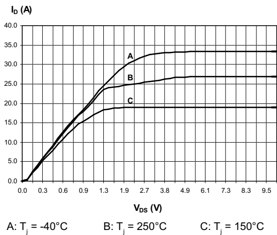
Figure 12. Output characteristics
