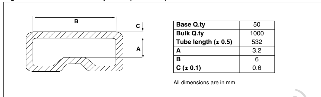
Figure 32. SO-16 tube shipment (no suffix)
