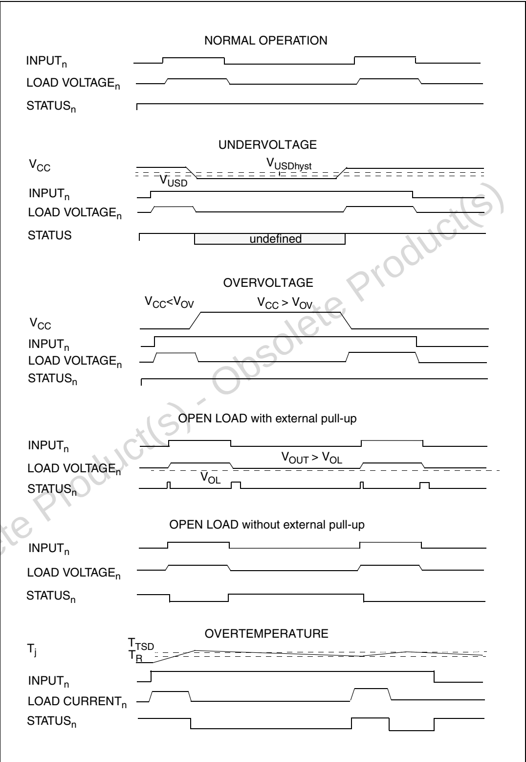
Figure 6. Waveforms
