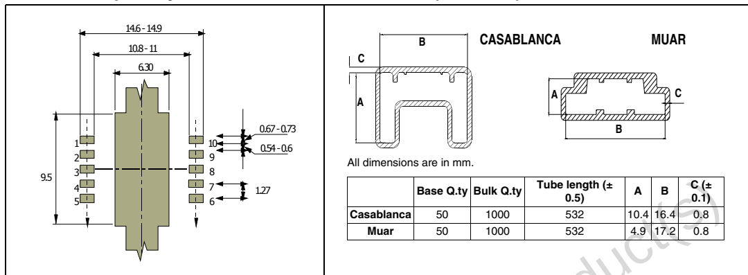
Figure 26. PowerSO-10 suggested pad layout
