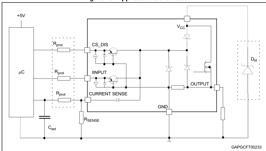
Figure 29. Application schematic
