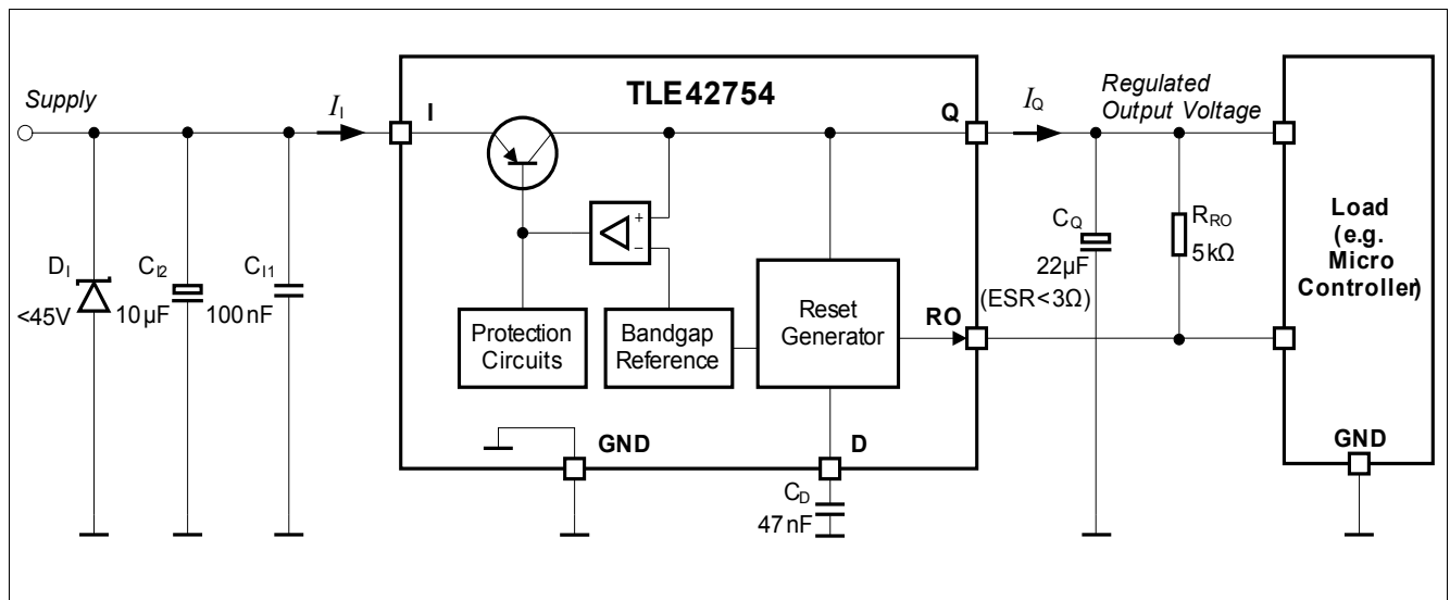
Figure 7 Application Diagram
