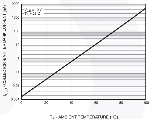
Figure 12. Dark Current vs. Ambient Temperature
