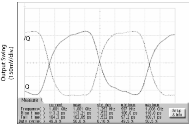
1GHz Output
