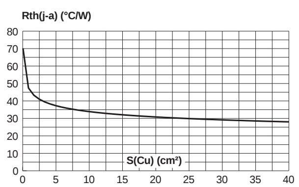
Fig. 10: Thermal resistance junction to ambient versus copper surface under tab (Epoxy printed circuit board, copper thickness: 35 \mu m ).
