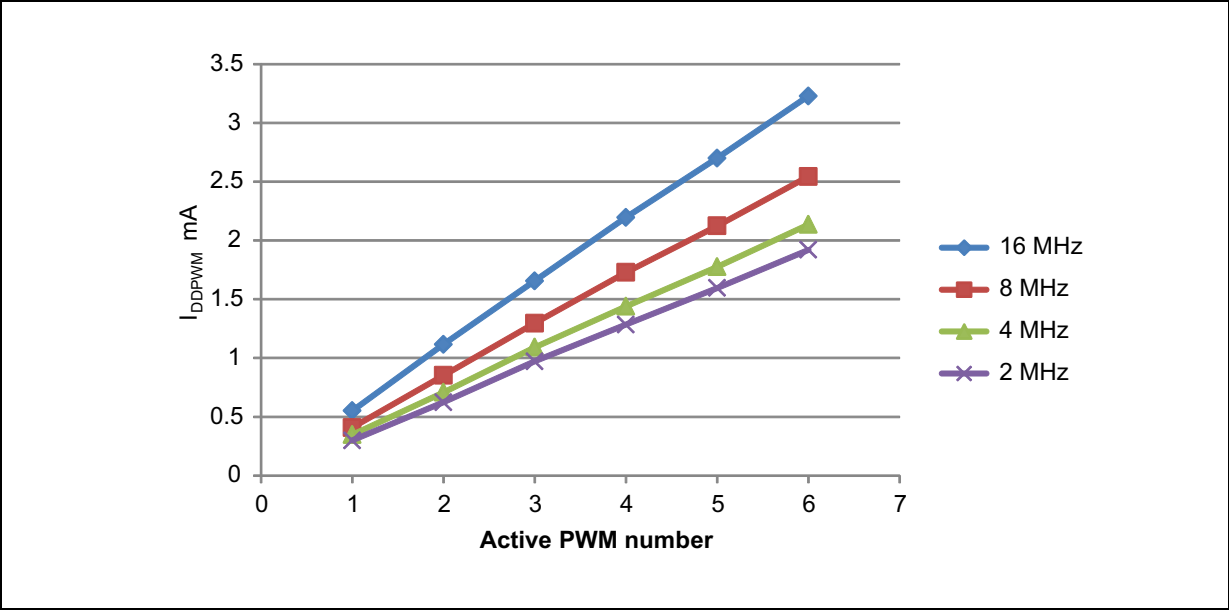
Figure 15. PWM current consumption with f_{SMED} = HSI f_{PWM} = 0.5 MHz at V_{DD}/V_{DDA} = 3.3 V
