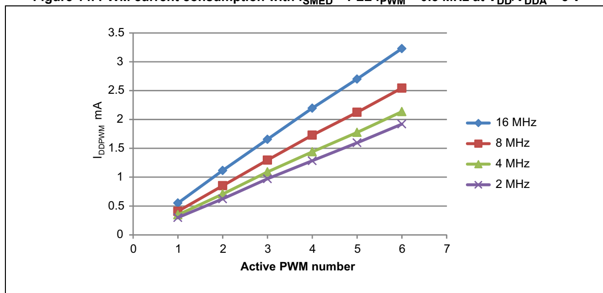
Figure 14. PWM current consumption with f_{\text{SMED}} = \text{PLL} f_{\text{PWM}} = 0.5\text{ MHz} at V_{\text{DD}}/V_{\text{DDA}} = 5\text{ V}
