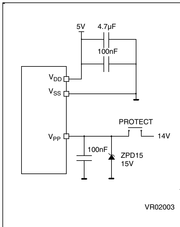
Figure 72. Programming Circuit
