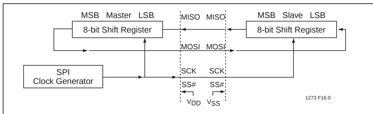
Figure 20: SPI Master-slave Interconnection
