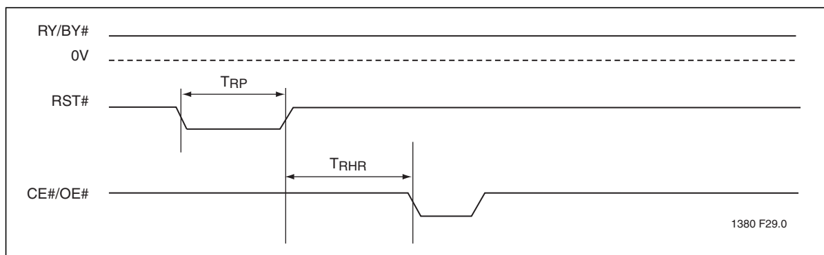
Figure 18: RST# Timing Diagram (When no internal operation is in progress)
