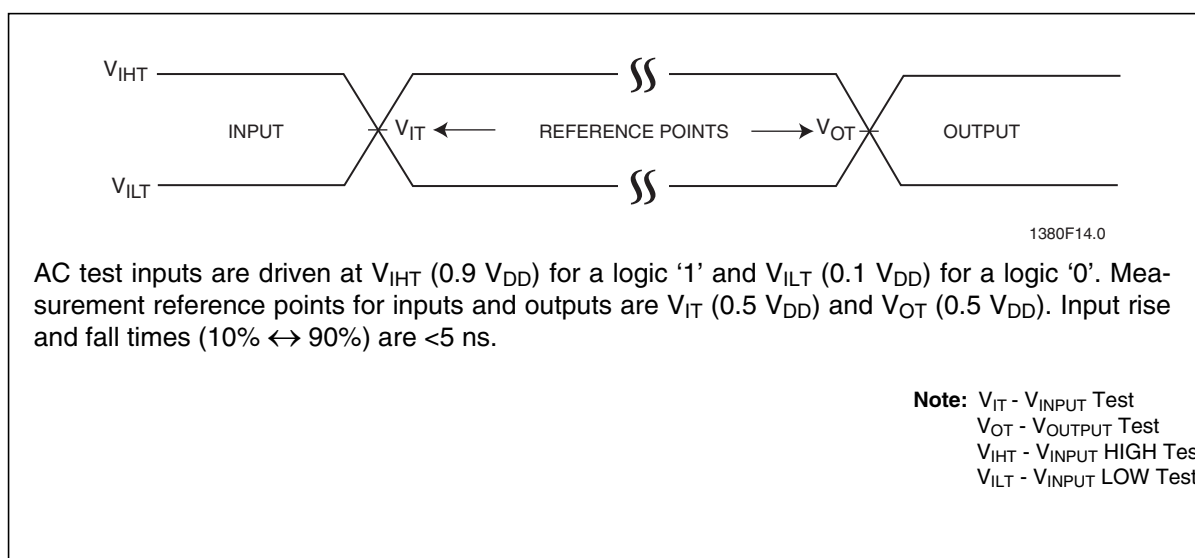
Figure 20: AC Input/Output Reference Waveforms
