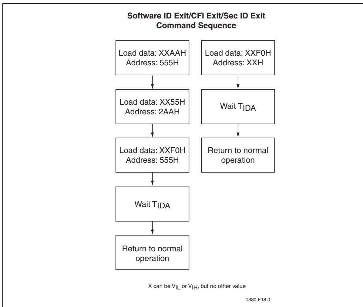
Figure 25: Software ID/CFI Exit Command Flowcharts
