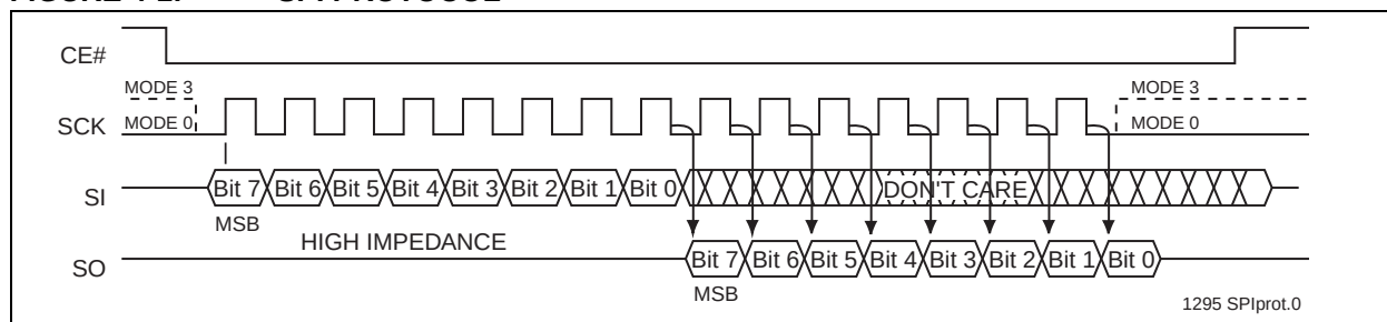
FIGURE 4-1: SPI PROTOCOL
