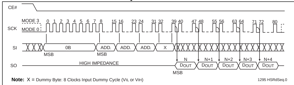
FIGURE 4-4: HIGH-SPEED-READ SEQUENCE
