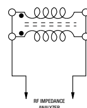
MEASURING CIRCUIT
