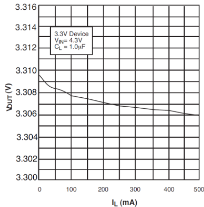
Fig. 8: Output Voltage vs Load Current
