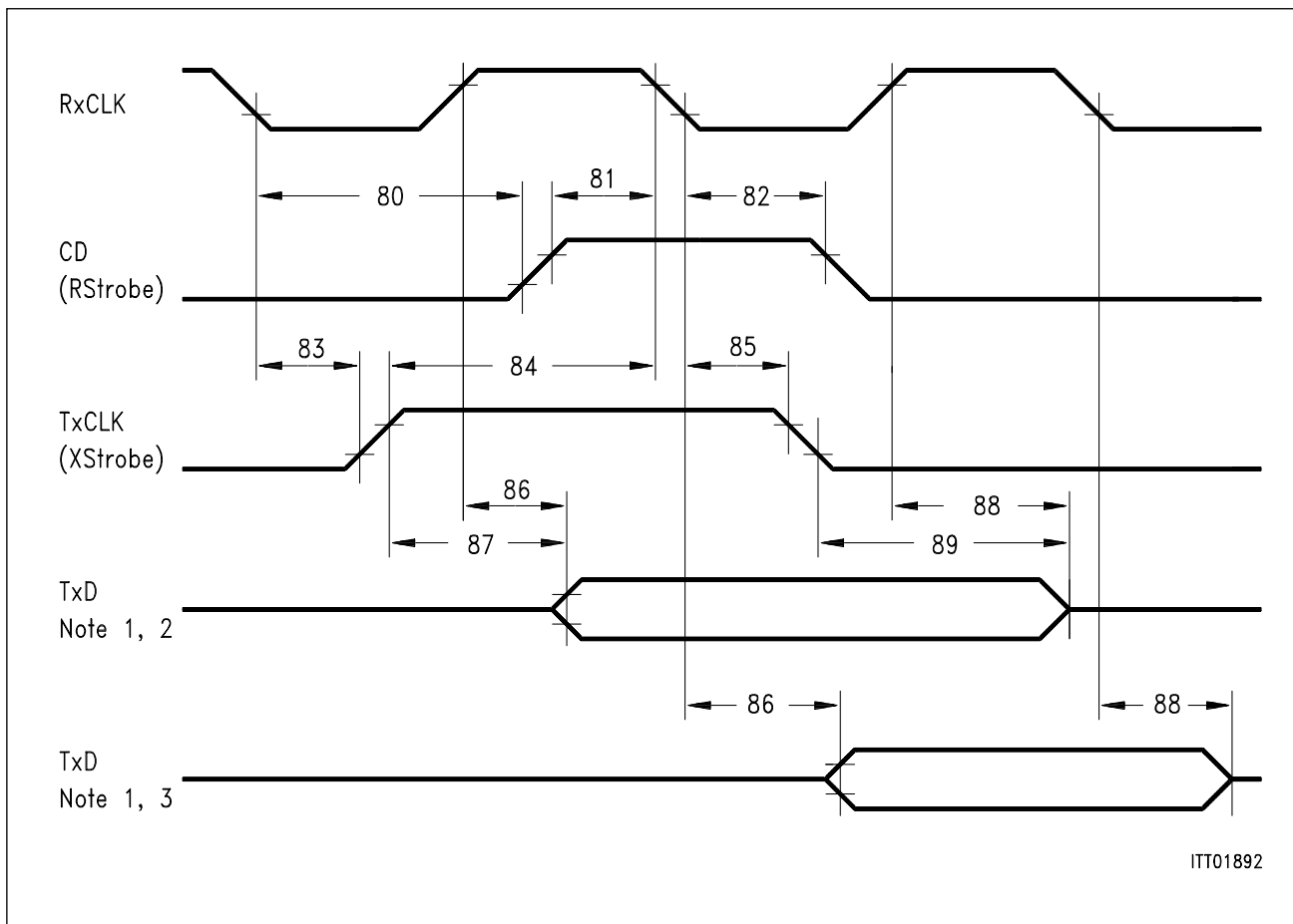
Figure 69 Strobe Timing
