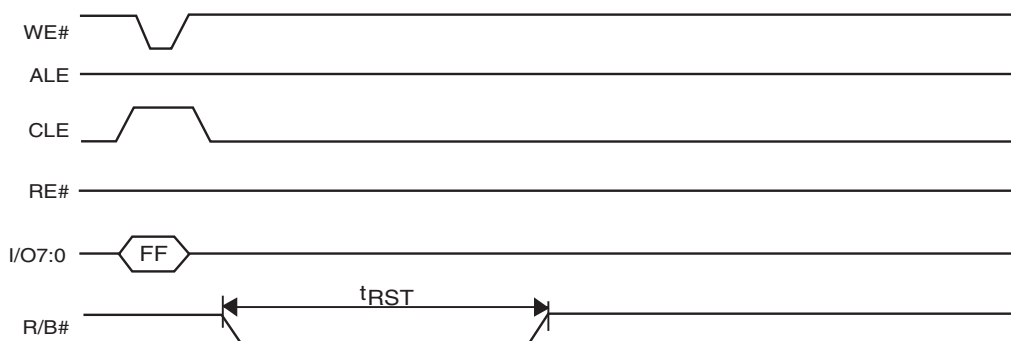
Figure 38. Reset Operation Timing
