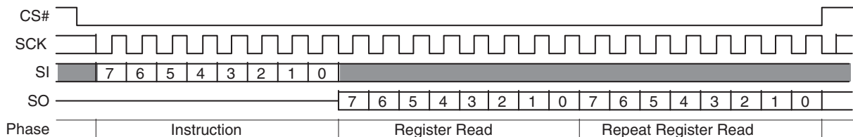
Figure 54. Read Configuration Register (RDRCR) Command Sequence
