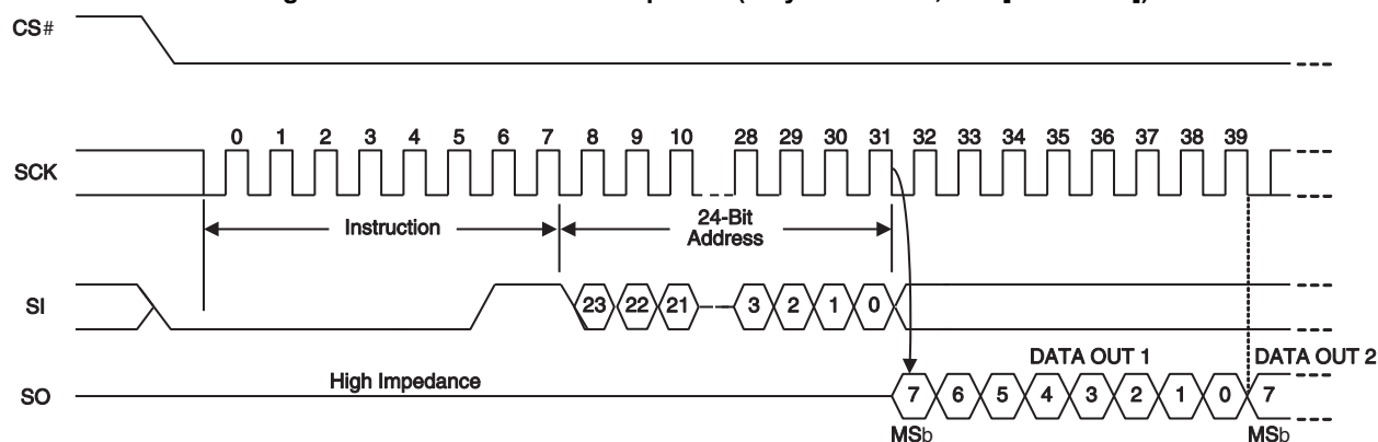
Figure 71. Read Command Sequence (3-byte Address, 03h [ExtAdd=0])
