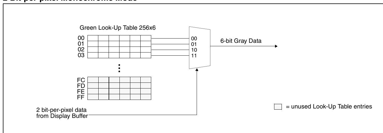
Figure 11-2: 2 Bit-per-pixel Monochrome Mode Data Output Path
