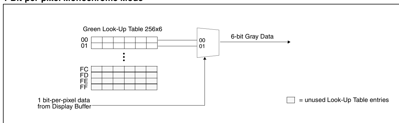
Figure 11-1: 1 Bit-per-pixel Monochrome Mode Data Output Path
