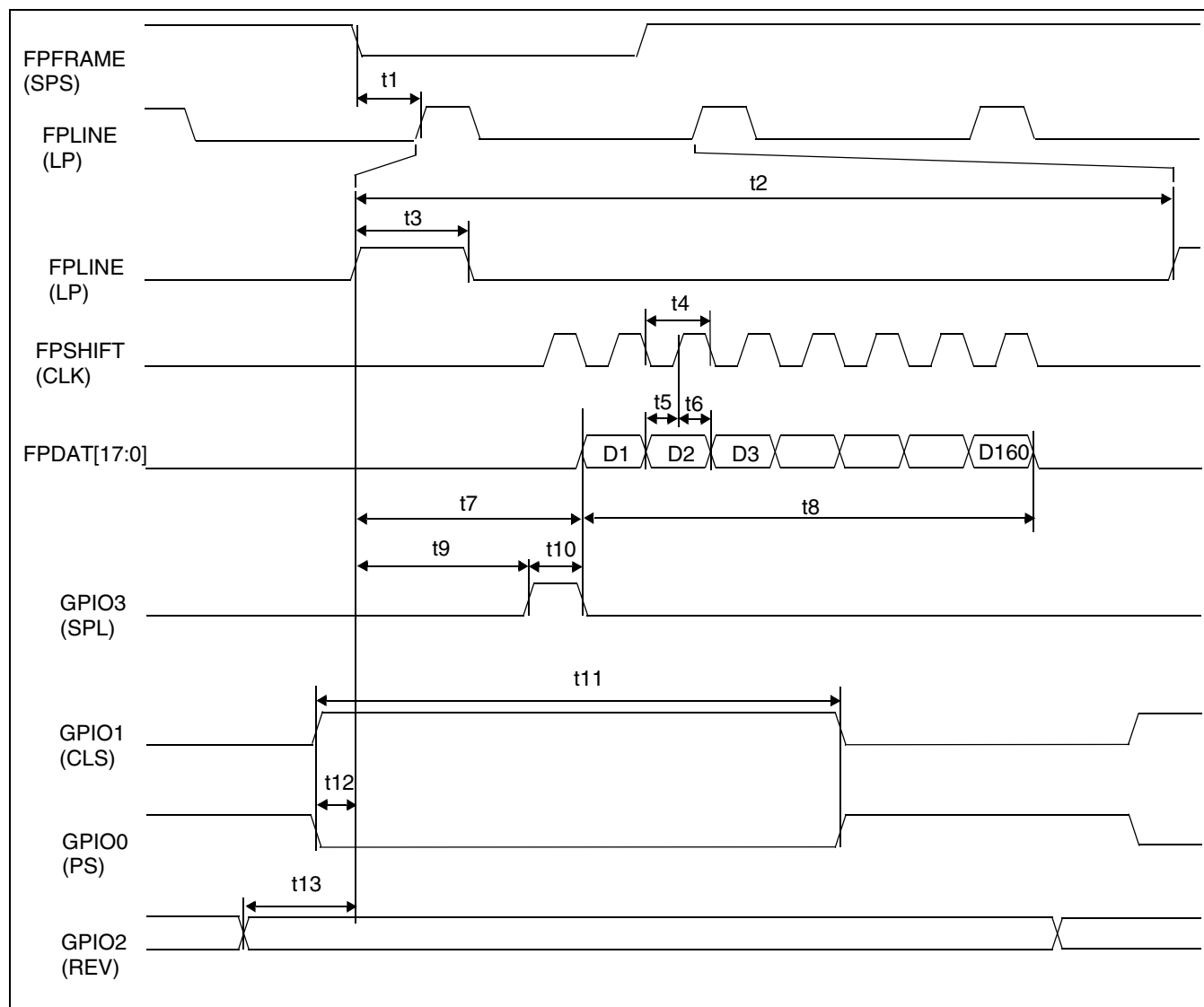
Figure 6-30: 160x160 Sharp 'Direct' HR-TFT Panel Horizontal Timing
