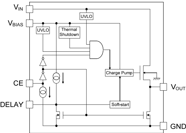
R5541K001D Block Diagram
