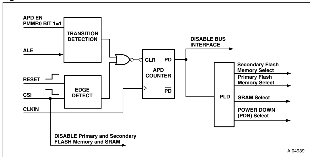
Figure 31. APD unit
