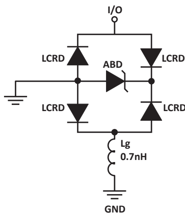
FIGURE 1 SPICE MODEL
