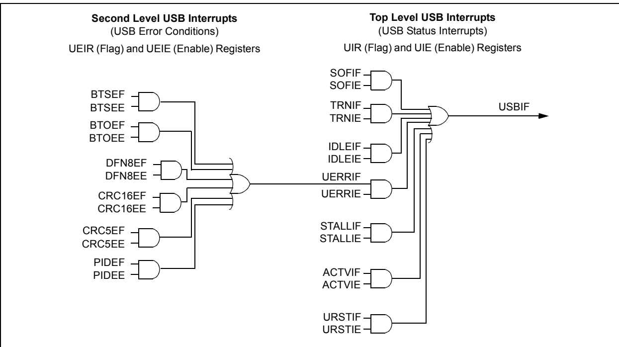
FIGURE 14-8: USB INTERRUPT LOGIC FUNNEL
