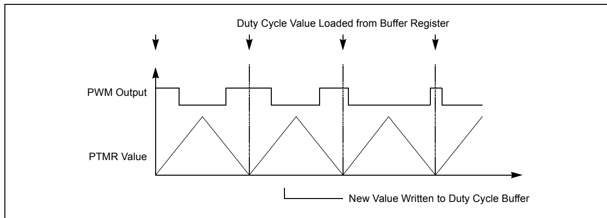
FIGURE 14-13: DUTY CYCLE UPDATE TIMES IN CONTINUOUS UP/DOWN COUNT MODE
