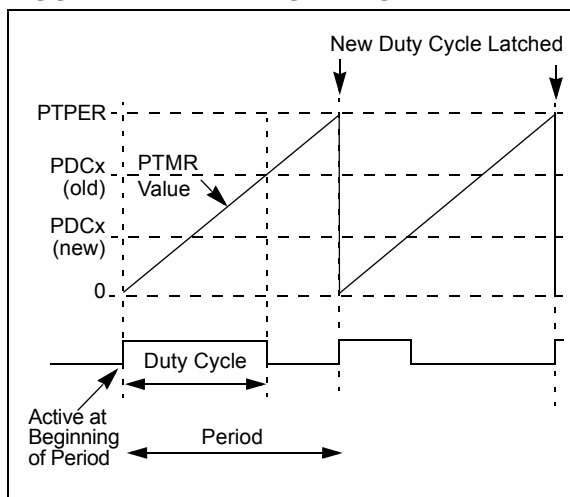
FIGURE 14-12: EDGE-ALIGNED PWM
