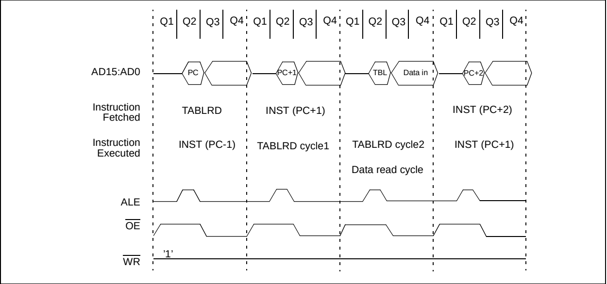
FIGURE 8-7: TABLRD TIMING
