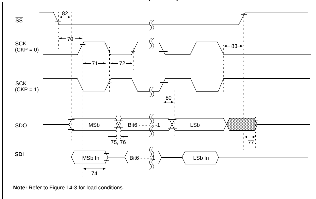
FIGURE 14-13: SPI SLAVE MODE TIMING (CKE = 1)
