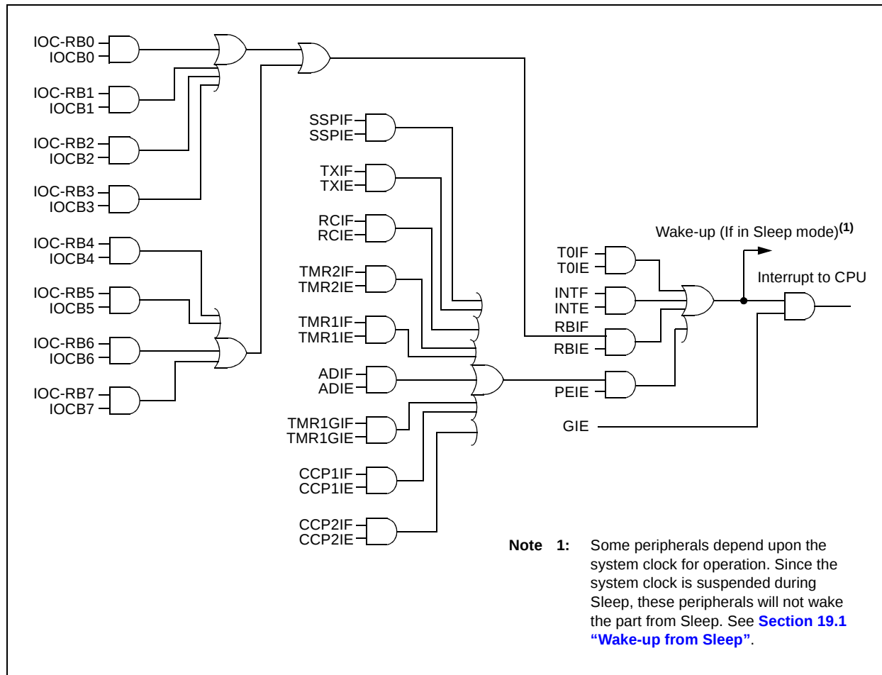
FIGURE 4-1: INTERRUPT LOGIC
