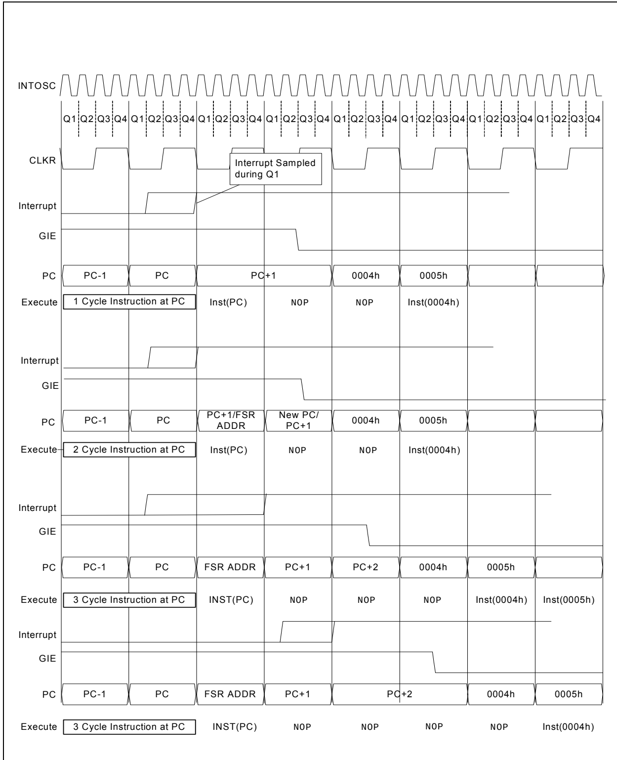
FIGURE 6-2: INTERRUPT LATENCY
