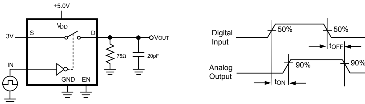
Figure 4. Switching Time
