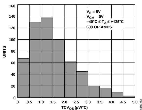
Figure 8. OP492 Temperature Drift ( TCV_{OS} ) Distribution @ 5 V
