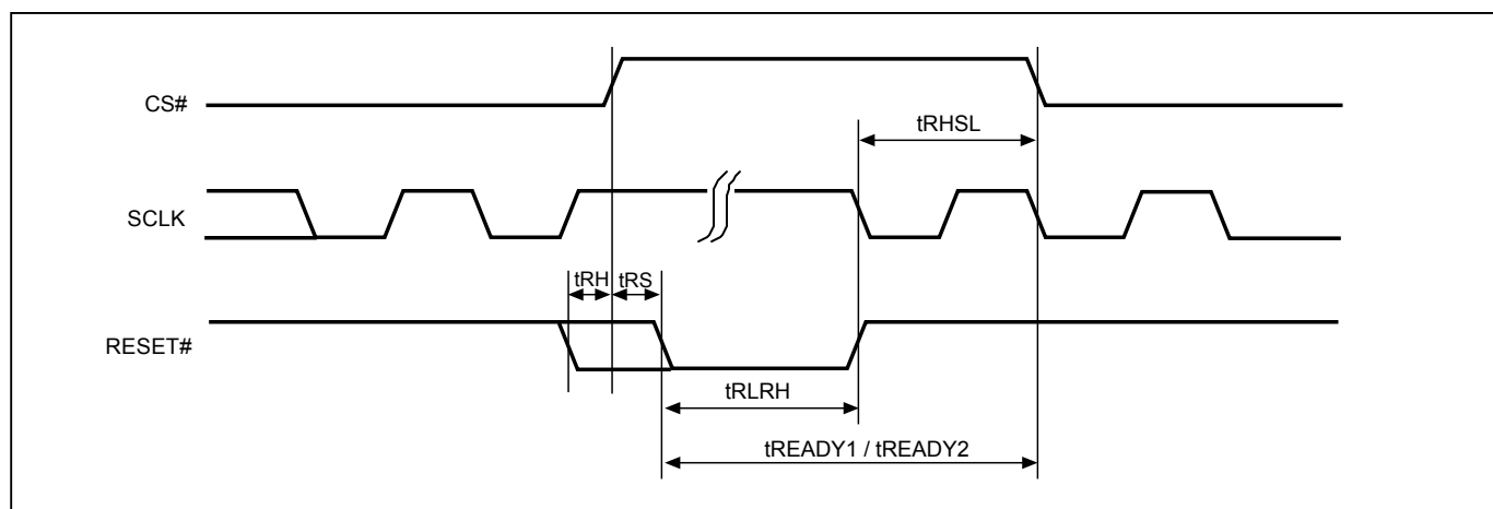
Figure 76. RESET Timing
