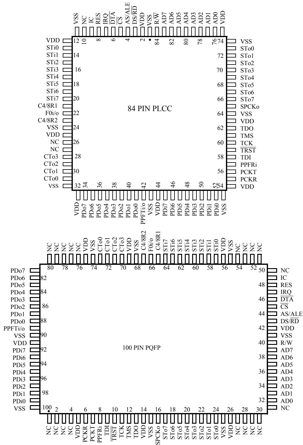
Figure 2 - Pin Connections
