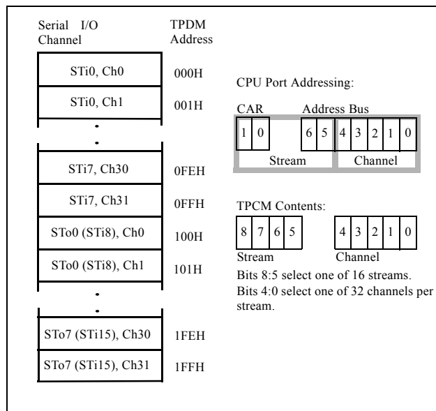
Figure 12a - 2.048 Mbps Add/Drop Mode TPDM Addressing
