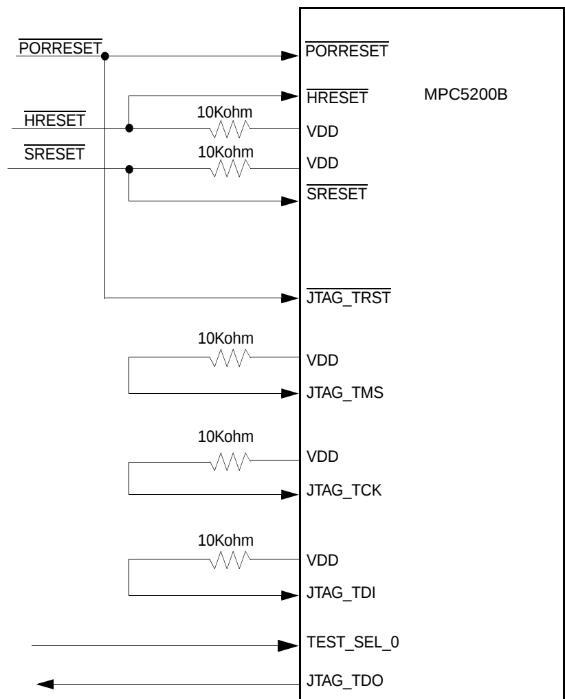
Figure 55. JTAG_TRST Wiring for Boards without COP Connector
